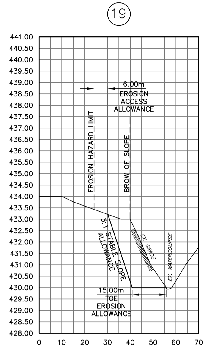
CROSS SECTIONS SCALE: HOR. 1:1000 VER. 1:100
